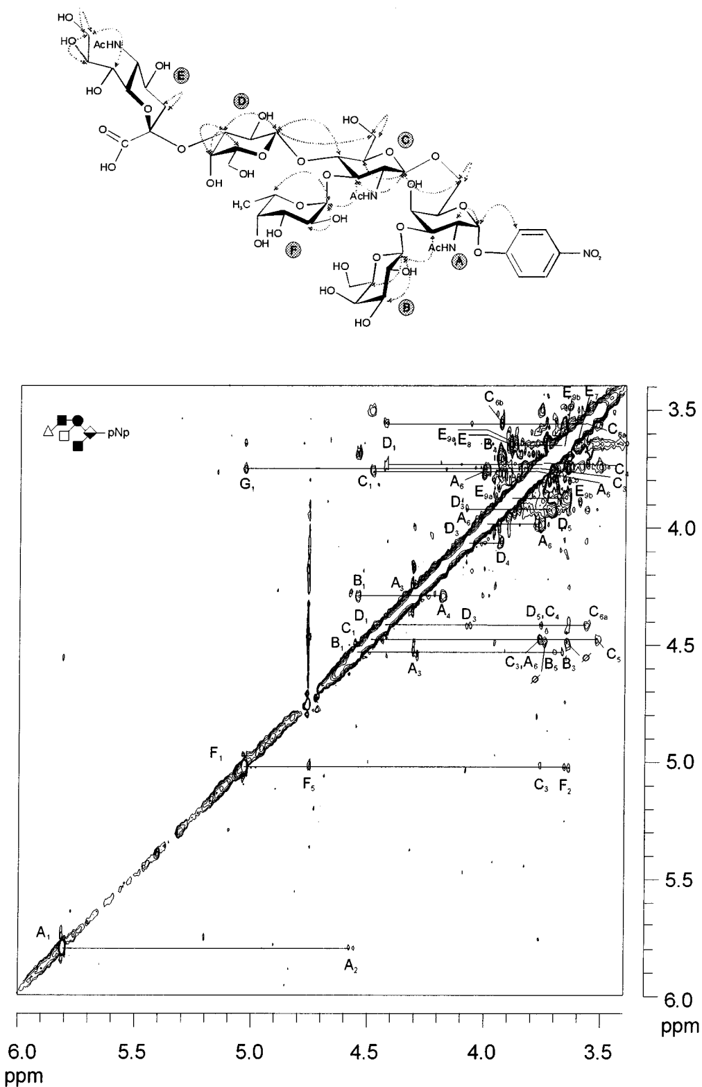
Figure 3. Two-dimensional 600 MHz ROESY spectrum (mixing time 200 ms) of Neu5Ac(α2-3)Gal(β1-4)[Fuc(α1-3)]GlcNAc(β1-6)[Gal(β1-3)]GalNAc(α1-pNp) (5) in 2 H 2 O at 300 K (referenced to internal acetone (δ 2.225)).
